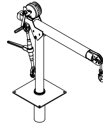
ISOMETRIC VIEW
