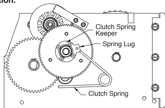
Clutch Spring Illustration
