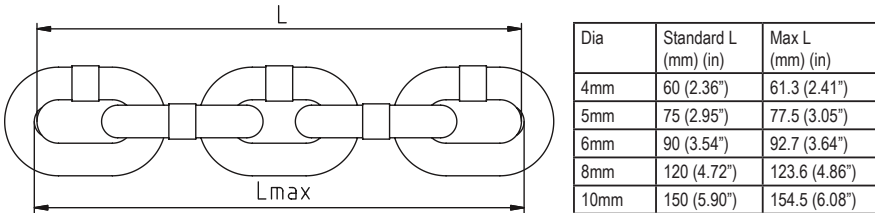
Load Chain - Five link length
