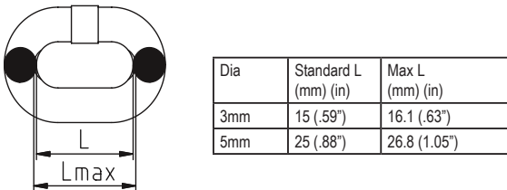
Hand Chain - One link length
